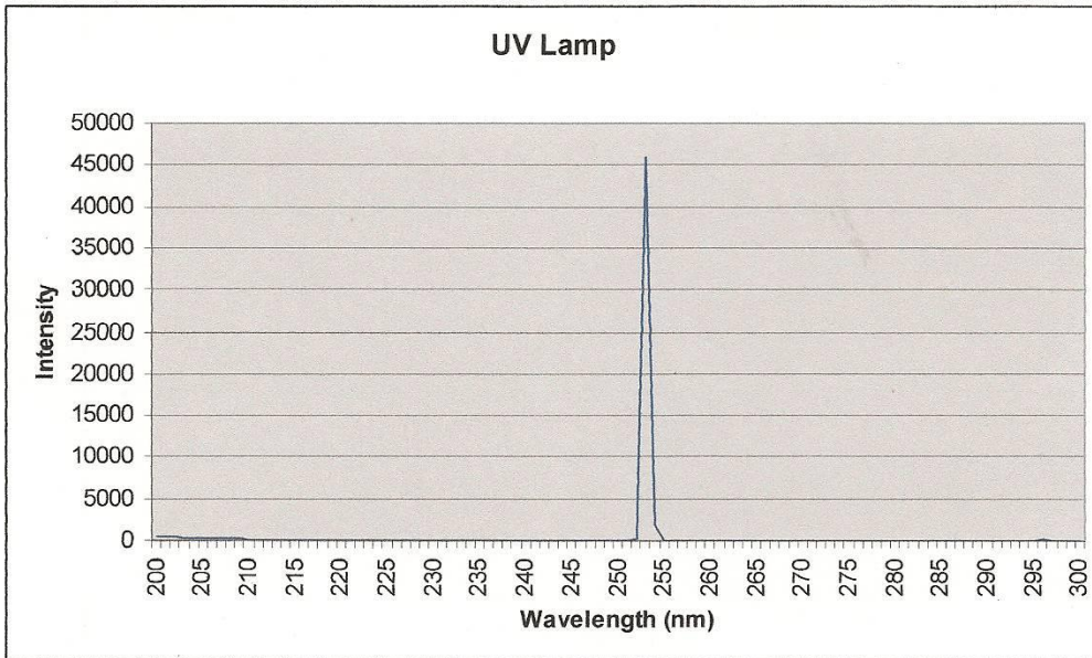
Chart 2 UV Tube Lamp 253nm
