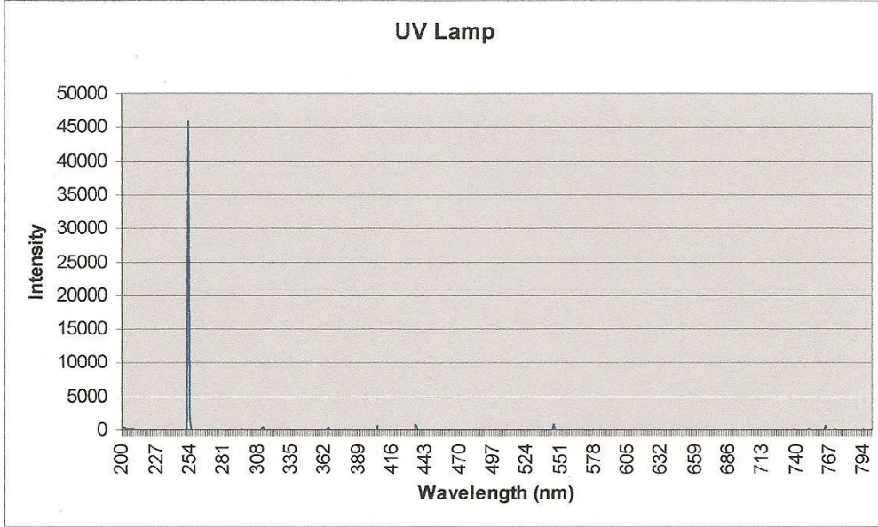
Chart 1 UV Tube Lamp 253nm
